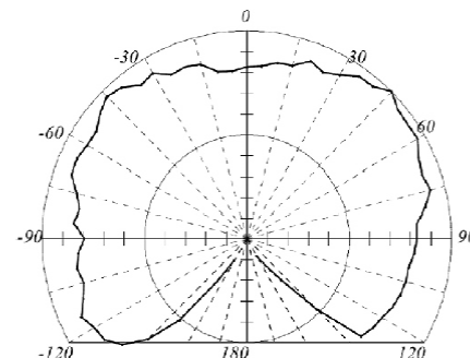
Incandescent Light Intensity Distribution Curve
