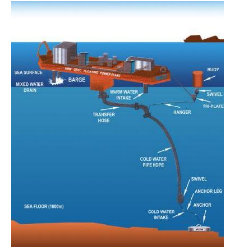
Ocean Thermal Energy Conversion
