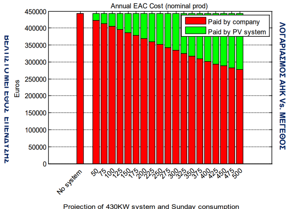
Projection of 430KW system and Sunday consumption
